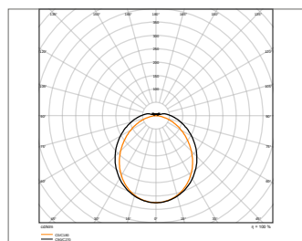
DP FLEX TH 1200 P 34W ML 830 IP66
