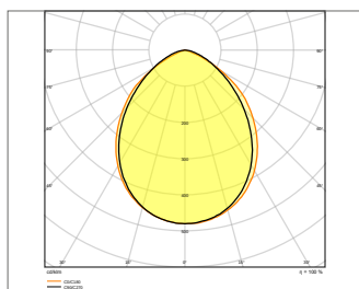
FL COMP SEN V 10W 830 SYM 100 BK
