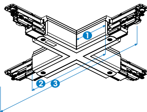
Middle feed XTSNC 614 1. 150 mm, 2. 280 mm
