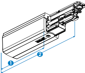
End feed XTSC 611, 612 1. 90 mm, 2. 155 mm
