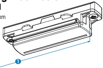
Adjustable corner connector GB 24 1. 100 mm, 2. 165 mm
